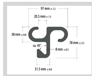
VTS Junction - 17,6 kg/m
