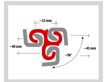
VT Junction - 18 kg/m
